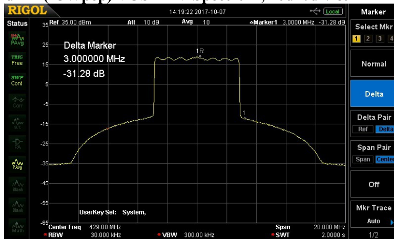
+40dBm (10 Watts rms), DVB-T Spectrum, 10dB/div & 2 MHz/div
