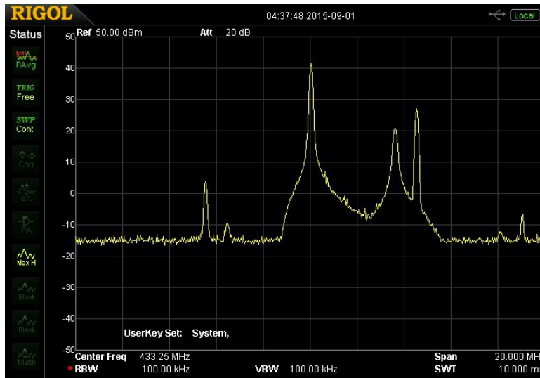
+44 dBm (25Wpep) VUSB-TV Spectrum, 10dB/div & 2 MHz/div
