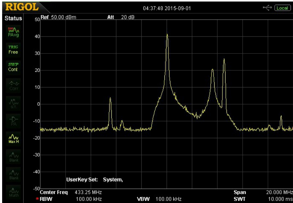
+43 dBm (20Wpep) VUSB-TV Spectrum, 10dB/div & 2 MHz/div
