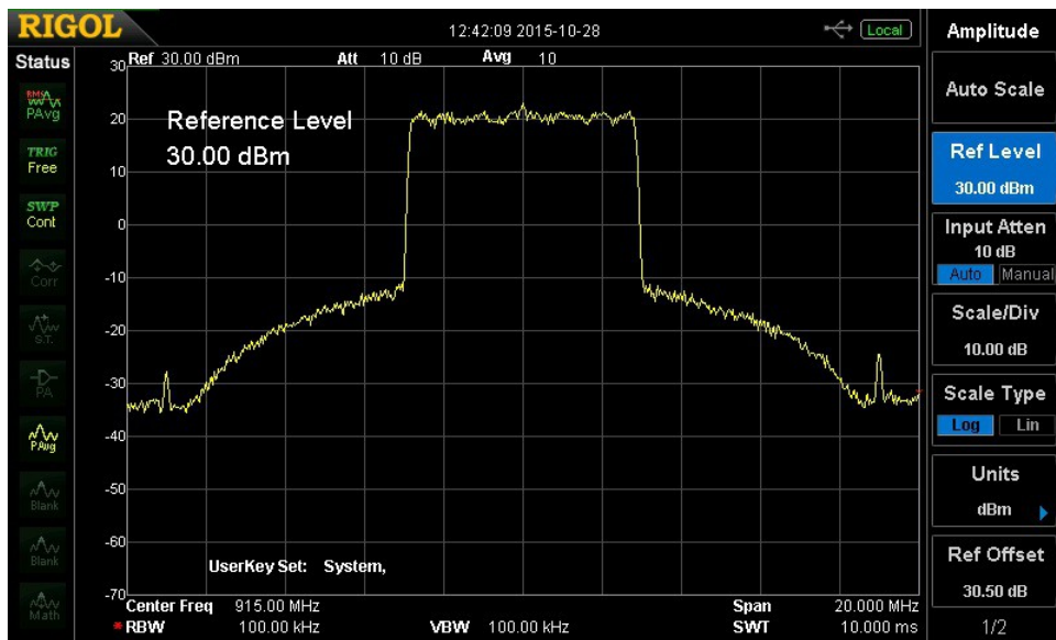
+38dBm (6 Watts rms), DVB-T Spectrum, 10dB/div & 2 MHz/div
