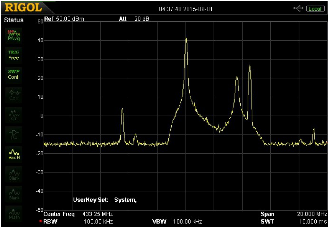
+44 dBm (25Wpep) VUSB-TV Spectrum, 10dB/div & 2 MHz/div (shown with NTSC color bars as test signal)
